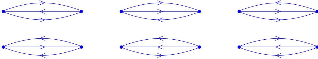
The six ways to make the \theta -graph into an oriented stratified-smooth space.
