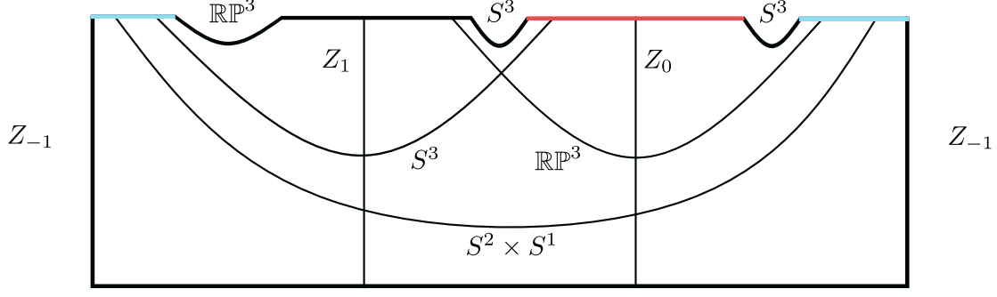
FIGURE 2. A representation of the cobordism W_{-1}^2 , with its five boundary components labeled. The more thin arcs represent the five submanifolds used in the construction of the family of metrics G_{-1}^2 , and each arc is labeled by the diffeomorphism type of the corresponding submanifold. The surface \hat{c}_{-1}^2 is represented as the lighter blue curve; the surface \hat{c}_{-1}^2 is the union of the darker red and lighter blue curves. The middle end \mathbb{RP}^3 is drawn differently than the S^3 middle ends to make the asymmetry more apparent. The pictures for other W_{i-3}^i are similar; for instance, the bundle data can on W_{i-3}^i obtained by cyclically permuting the three depicted pieces.
